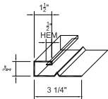
5 TYPICAL J-CHANNEL 3/4" = 1'-0"
