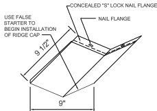
9 TYPICAL HIP & RIDGE CAP 1 1/2" = 1'-0"
