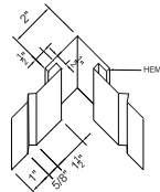
11 OUTSIDE CORNER FLASHING 3/4" = 1'-0"
