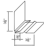
6 TYPICAL END WALL 3/4" = 1'-0" 8" WIDE SHEET BEFORE FOLDS
