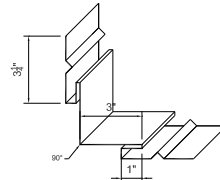
10 INSIDE CORNER FLASHING 3/4" = 1'-0"
